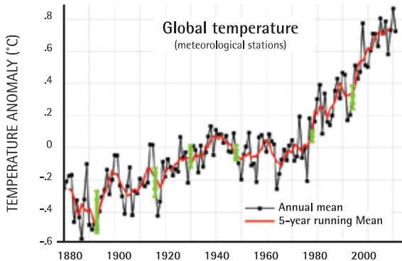
Figure 1. Global annual mean surface air temperature change: Uncertainty bars (95% confidence limits) are shown for both the annual and 5-year means and account only for incomplete spatial sampling of data.
